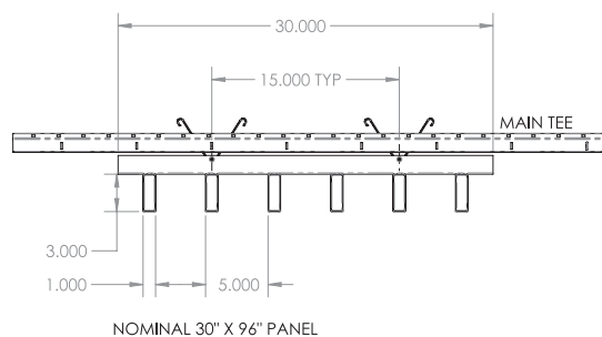
NUVO-Baffle Panel - TSP (30" X 96" module size shown)
