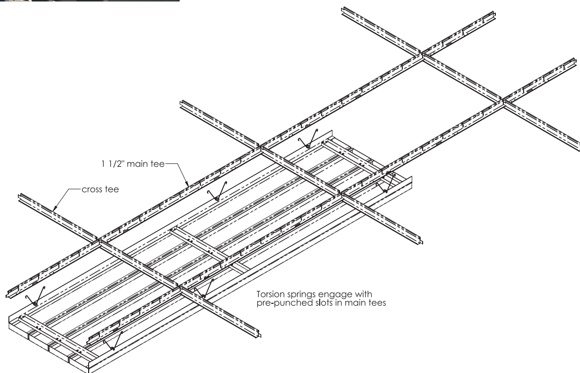
NUVO-Plank Panel TSP with suspension grid
