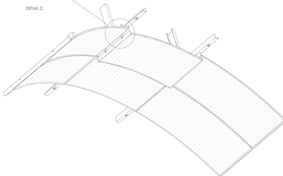
TYP. ISOMETRIC VIEW FROM BELOW
