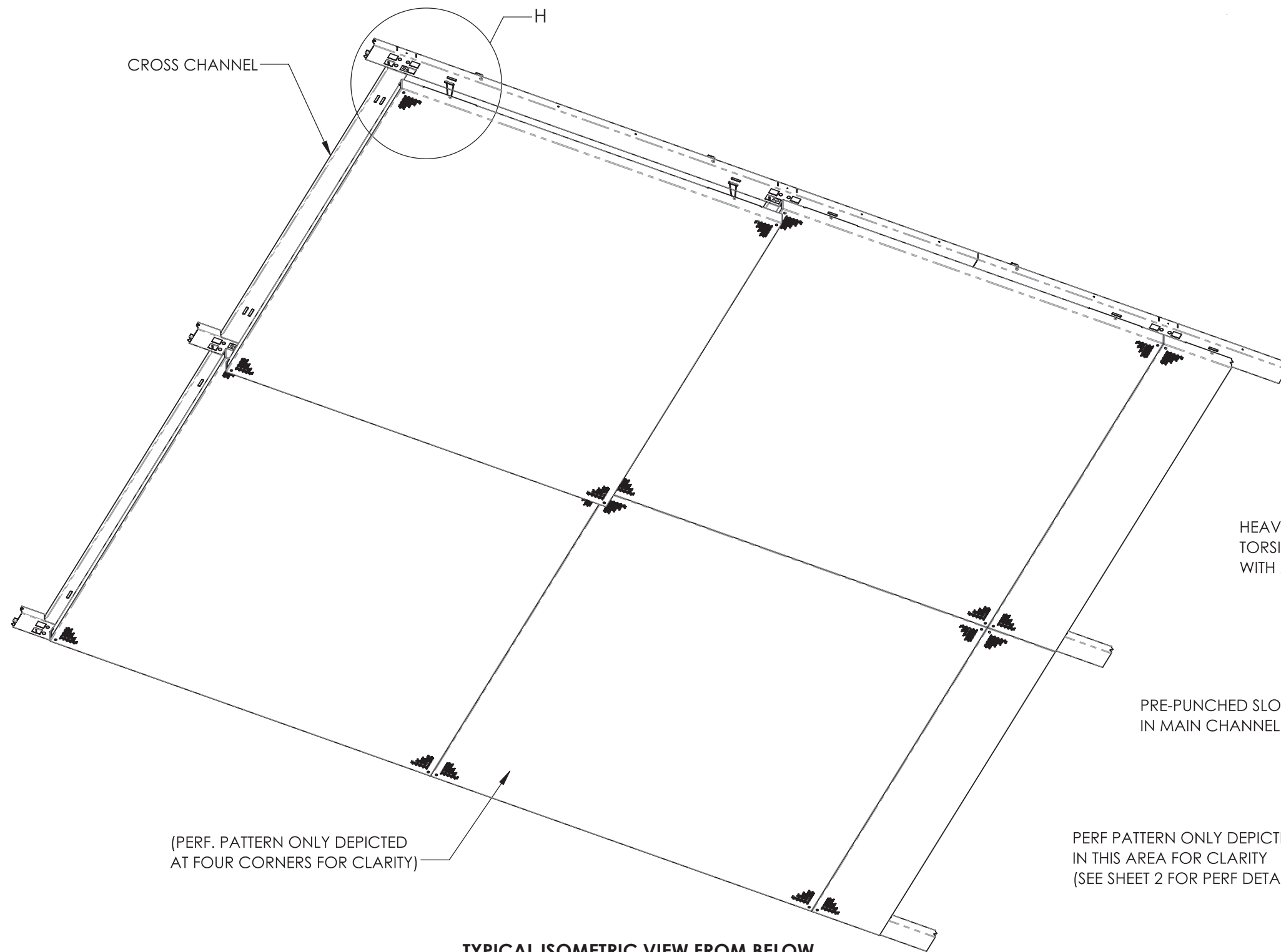
TYPICAL ISOMETRIC VIEW FROM BELOW
